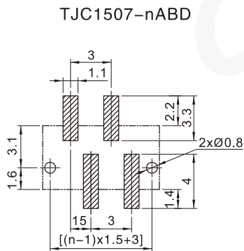
PCB Layout
