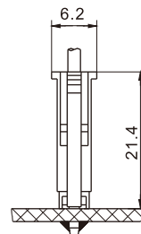
Assembly View (DIM FYI)
