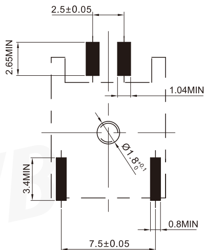
PCB Layout
